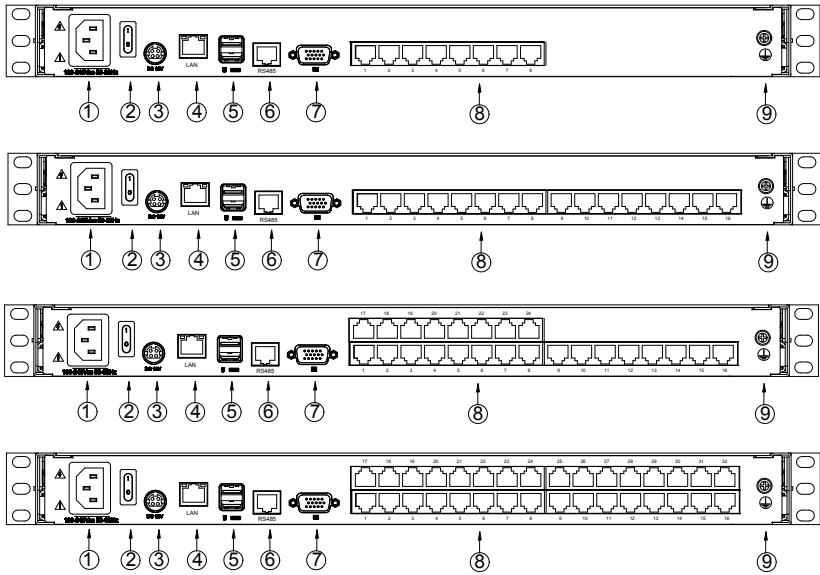
Figure 1.3 Rear view
