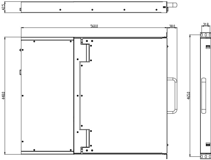
Figure 1.2 dimensions
