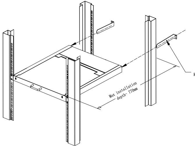
1-2.1 rack mounting (1)
