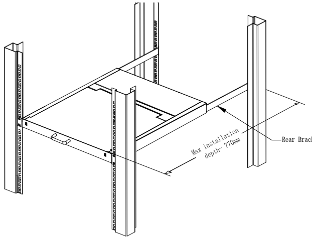
1-2.2 rack mounting (2)
