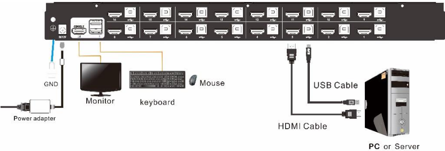
1.2 Installation Diagram
