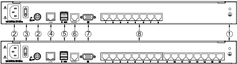
Figure 1.3 Rear view
