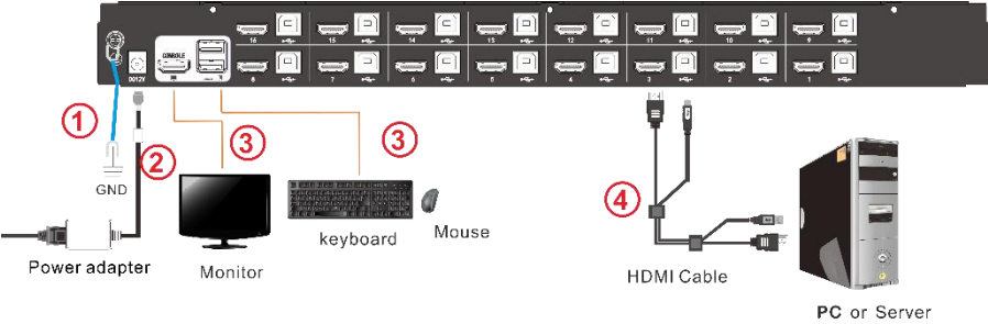
1.2 Installation Diagram
