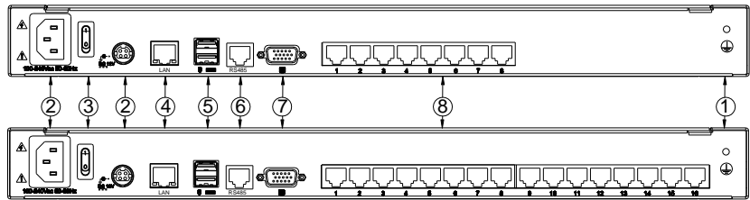
Figure 1.2 Rear view
