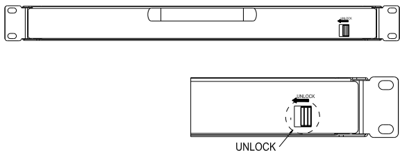
Figure 2.4 Unlocking
