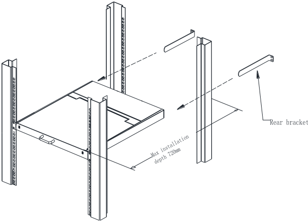
1-2.1 rack mounting (1)
