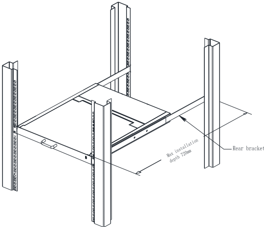
1-2.2 rack mounting (2)
