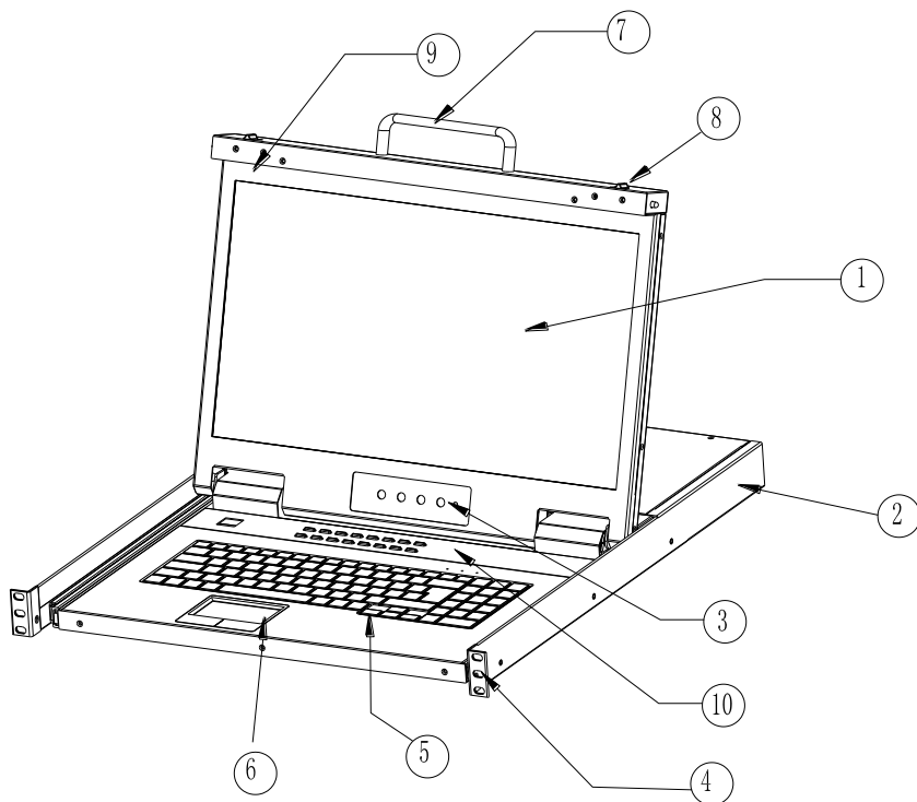
1-1.1 front view
