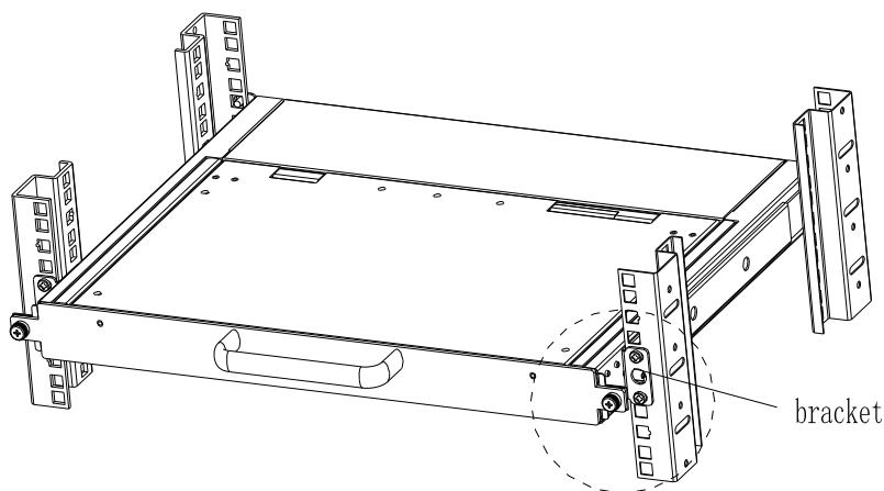
2-1.3 rack mounting (3)
