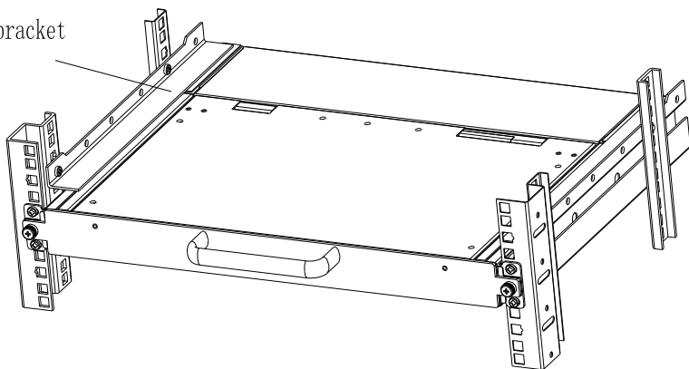
2-1.4 rack mounting (4)
