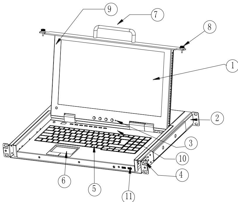
1-1.1 front view
