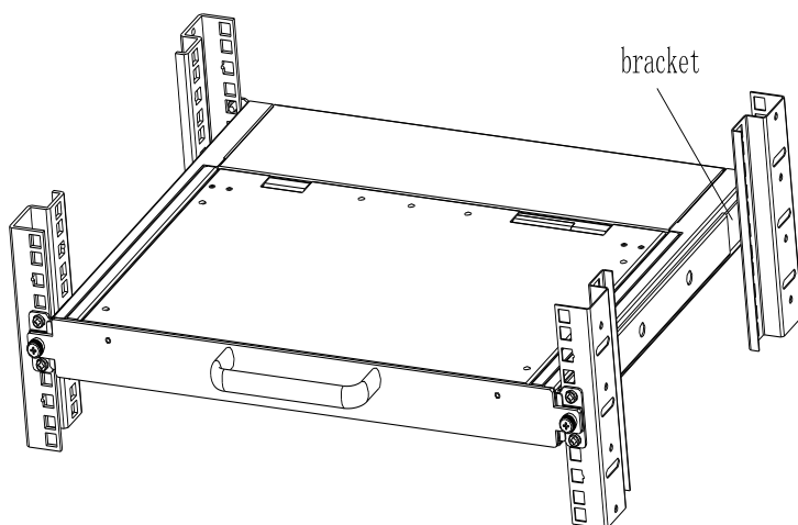
2-1.2 rack mounting (2)
