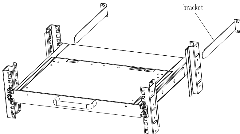
2-1.1 rack mounting (1)
